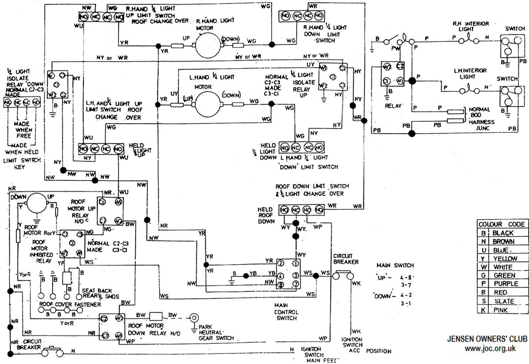
FIG. N16B - ROOF, 1/2 LIGHT AND INTERIOR LIGHT CIRCUIT UP TO CHASSIS No. 9490
