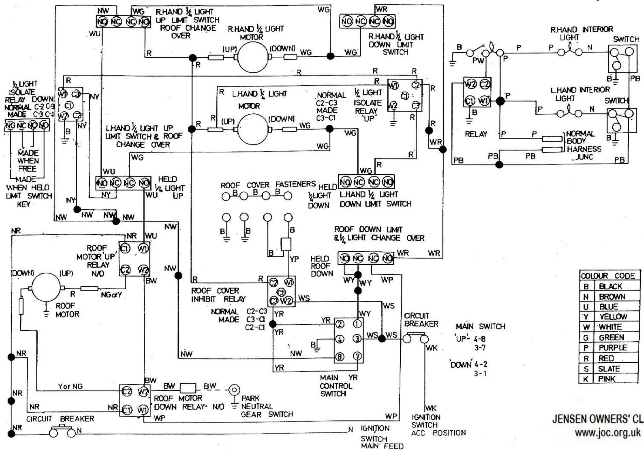
FIG. N14B ROOF 1/2 LIGHT AND INTERIOR LIGHT CIRCUIT FROM CHASSIS No. 9670
